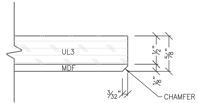
2 1.2 CHAMFER DETAIL SCALE: FULL
