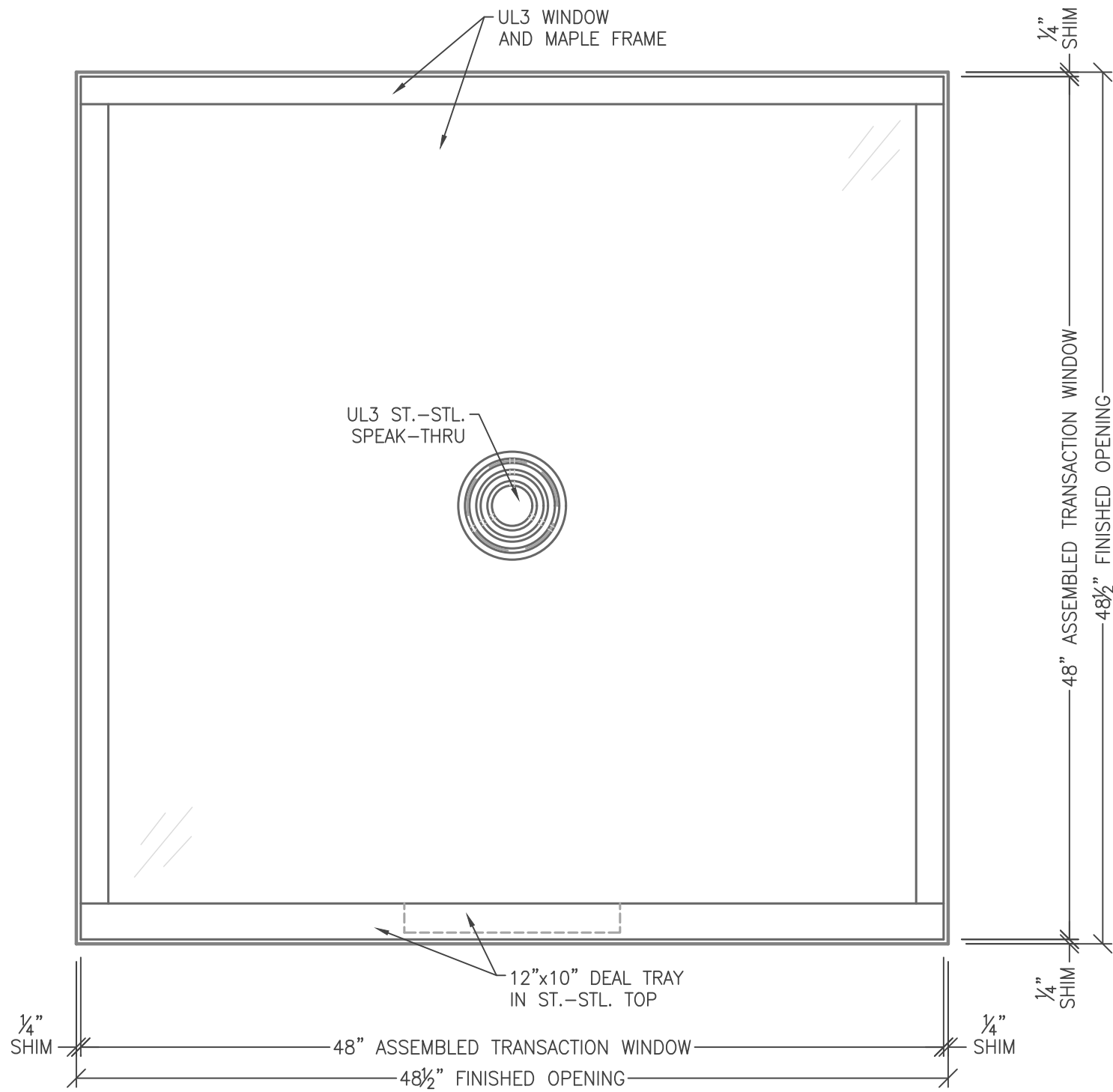
ATTACK SIDE ELEVATION 2 4.35 SCALE: 1-1/2" = 1'-0"
