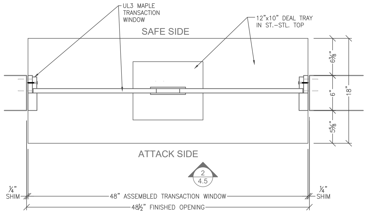
UL3 TRANSACTION WINDOW SPEAK THROUGH TW-ST-4040-MAP18-UL03 1 4.35 SCALE: 1-1/2" = 1'-0"
