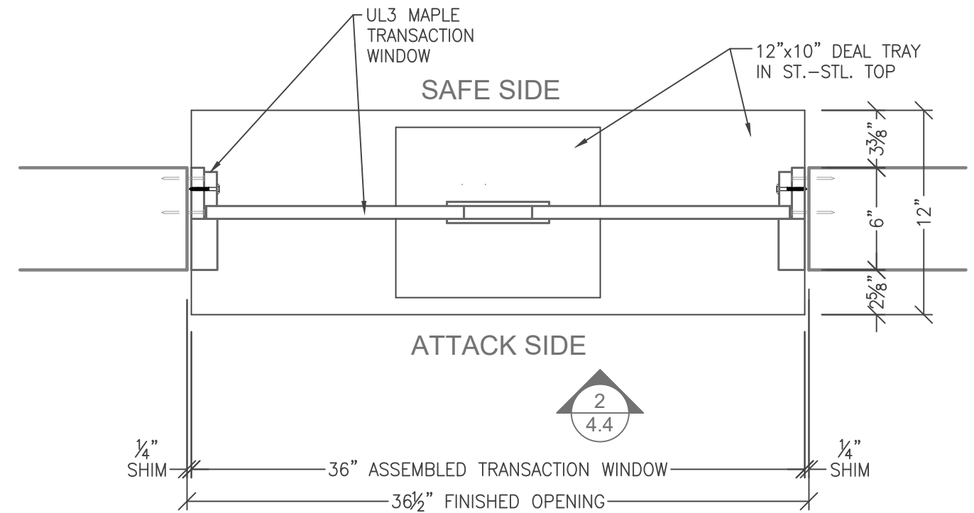
1 4.4 UL3 TRANSACTION WINDOW SPEAK THROUGH TW-ST-3040-MAP12-UL03 SCALE: 1-1/2" = 1'-0"
