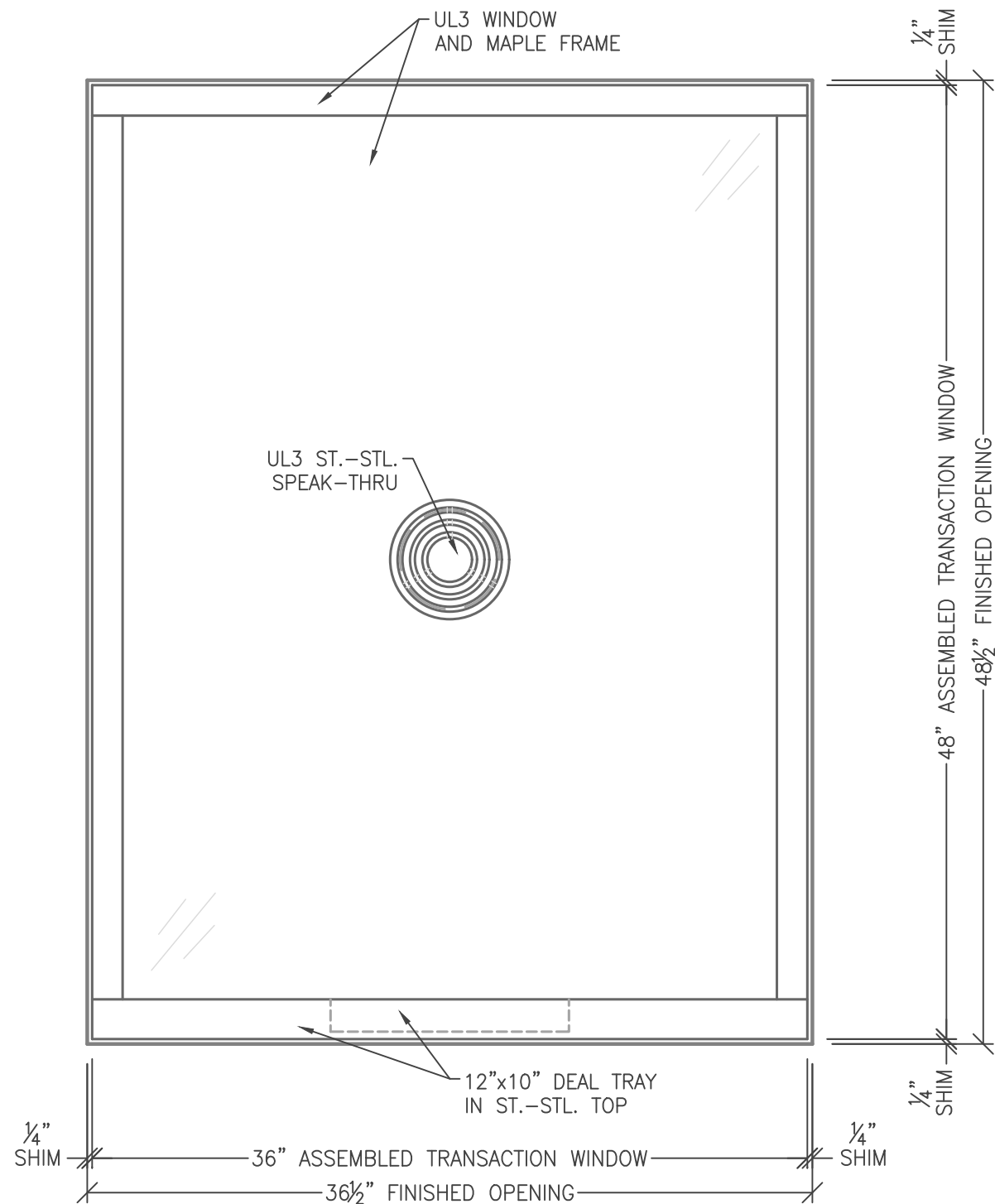
2 4.4 ATTACK SIDE ELEVATION SCALE: 1-1/2" = 1'-0"
