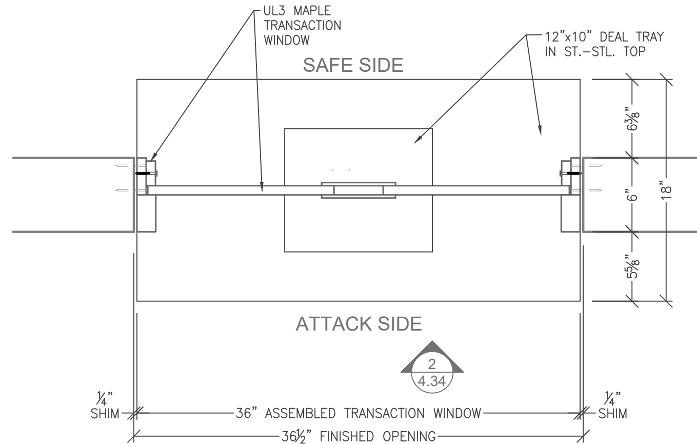
1 4.34 UL3 TRANSACTION WINDOW SPEAK THROUGH TW-ST-3040-MAP18-UL03 SCALE: 1-1/2" = 1'-0"
