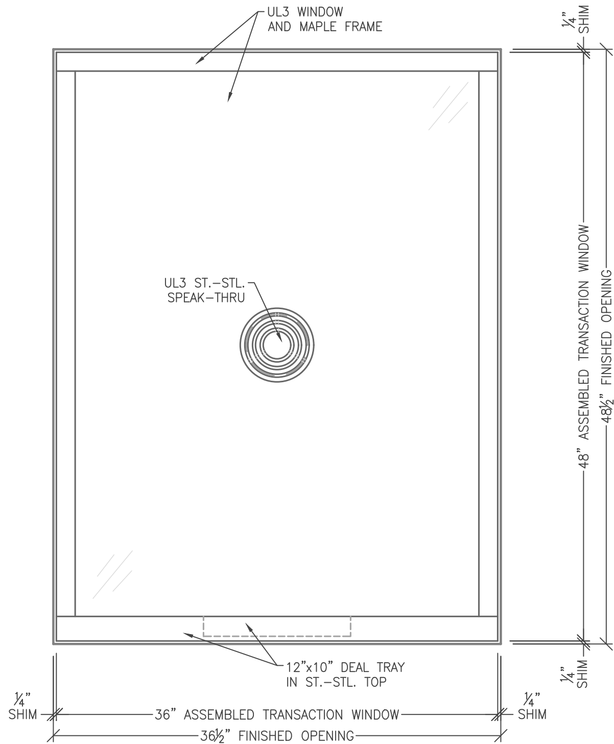
2 4.34 ATTACK SIDE ELEVATION SCALE: 1-1/2" = 1'-0"
