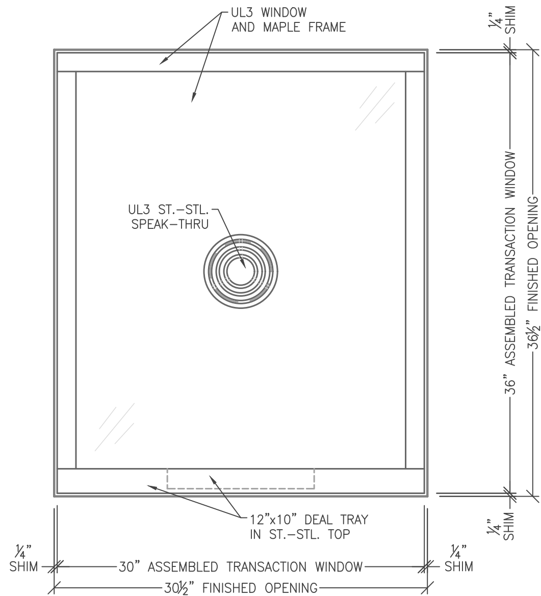
2 ATTACK SIDE ELEVATION 4.31 SCALE: 1-1/2" = 1'-0"
