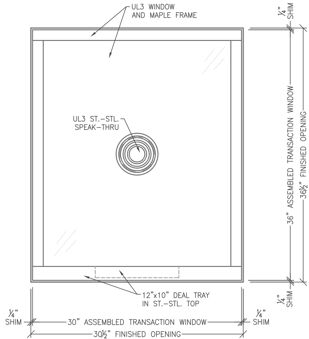
2 4.1 ATTACK SIDE ELEVATION SCALE: 1-1/2" = 1'-0"
