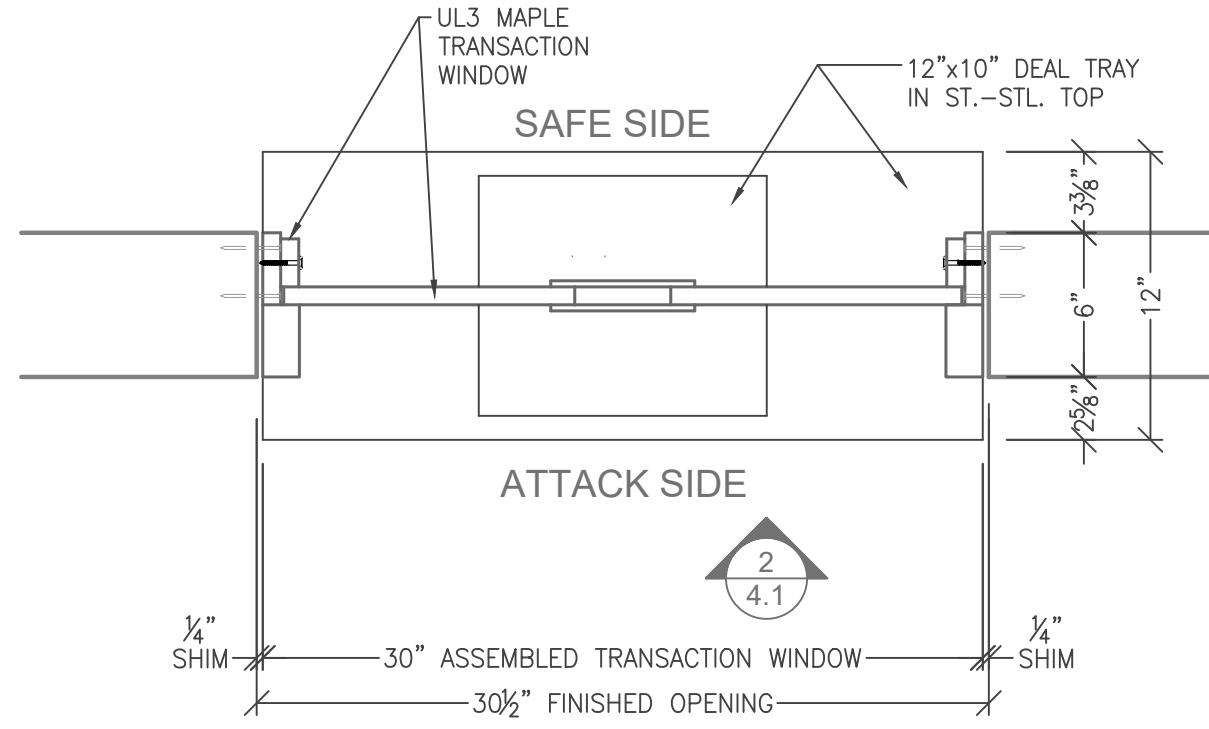
1 4.1 UL3 TRANSACTION WINDOW SPEAK THROUGH TW-ST-2630-MAP12-UL03 SCALE: 1-1/2" = 1'-0"
