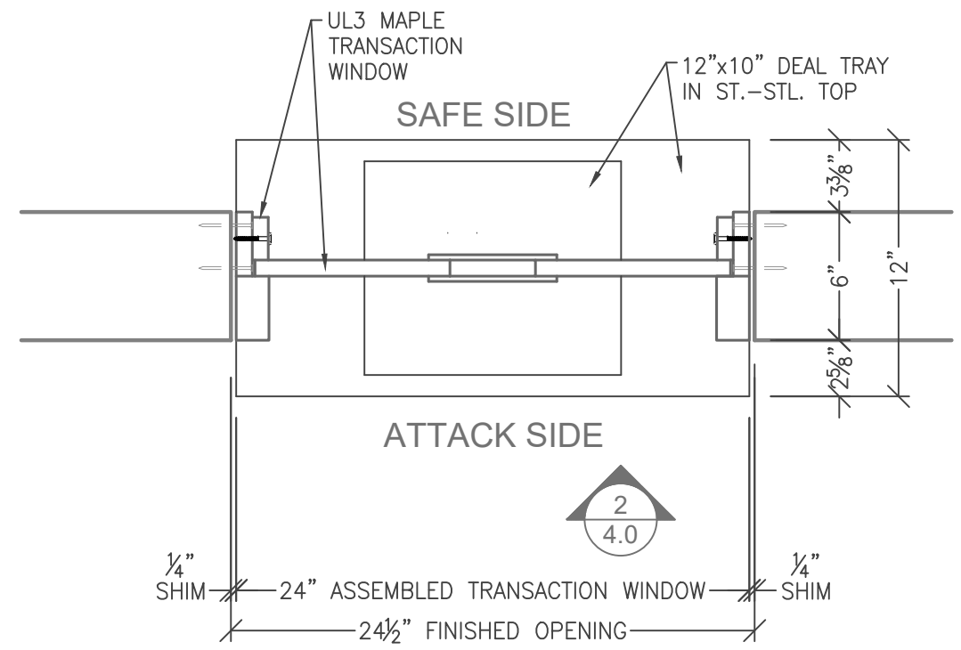
UL3 TRANSACTION WINDOW SPEAK THROUGH TW-ST-2030-MAP12-UL03 1 4.0 SCALE: 1-1/2" = 1'-0"
