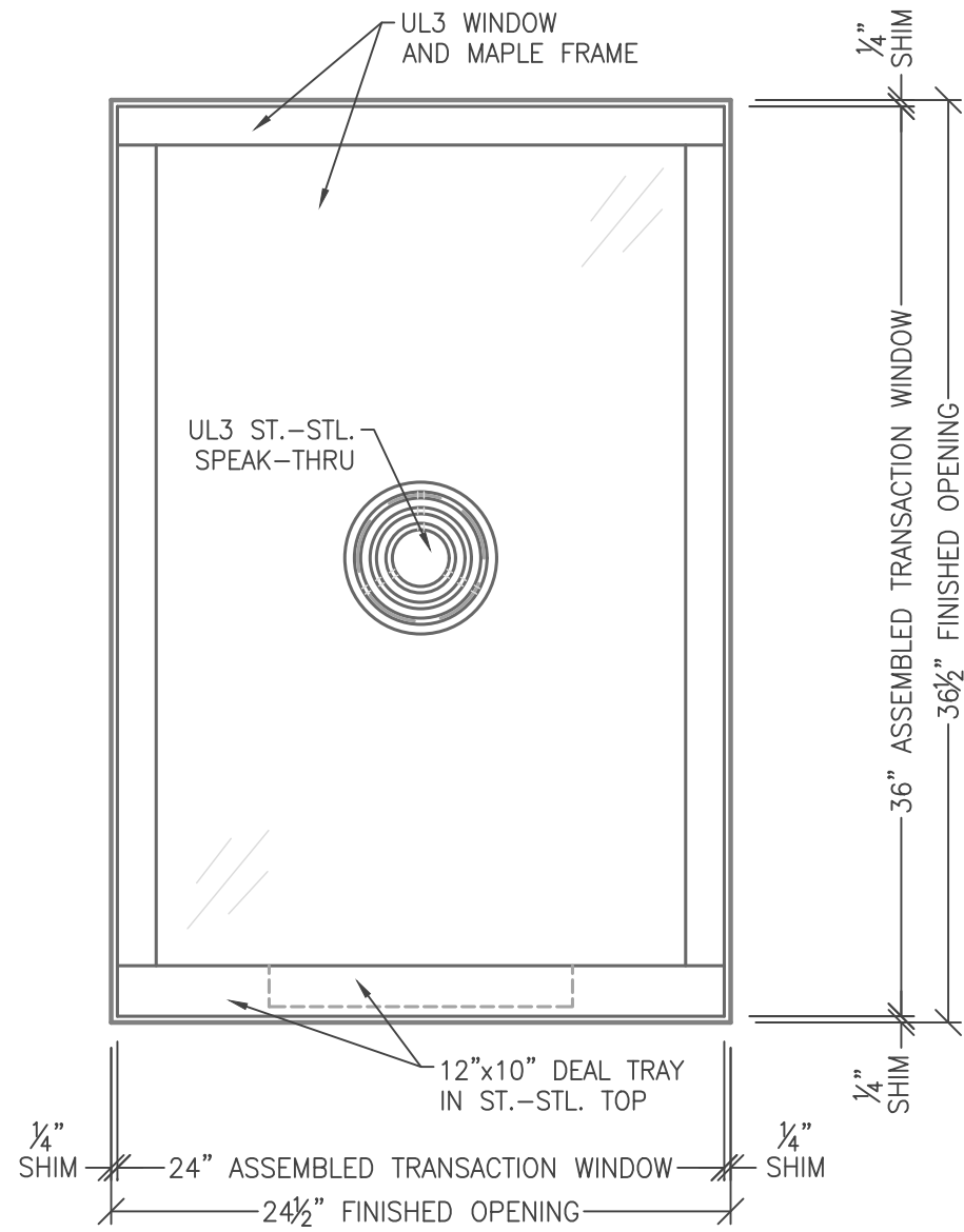
ATTACK SIDE ELEVATION 2 4.0 SCALE: 1-1/2" = 1'-0"
