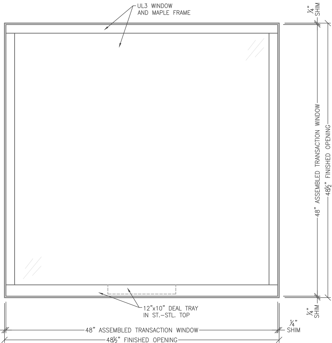
2 ATTACK SIDE ELEVATION SCALE: 1-1/2" = 1'-0"
