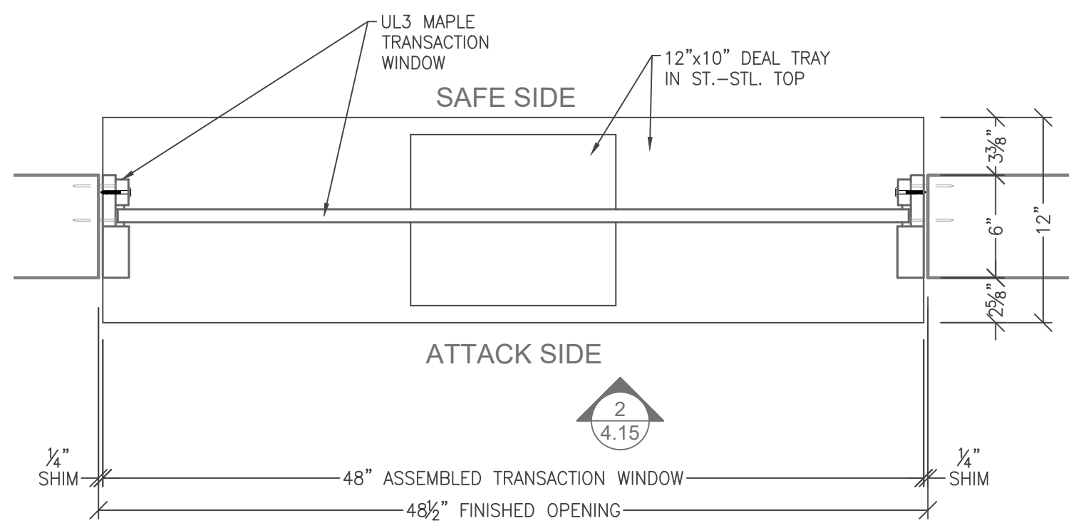
1 4.15 UL3 TRANSACTION WINDOW NATURAL VOICE TW-NV-4040-MAP12-UL03 SCALE: 1-1/2" = 1'-0"
