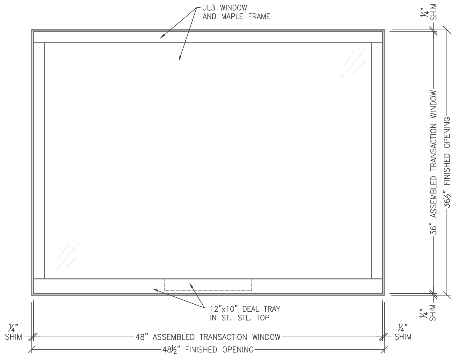
2 4.43 ATTACK SIDE ELEVATION SCALE: 1-1/2" = 1'-0"
