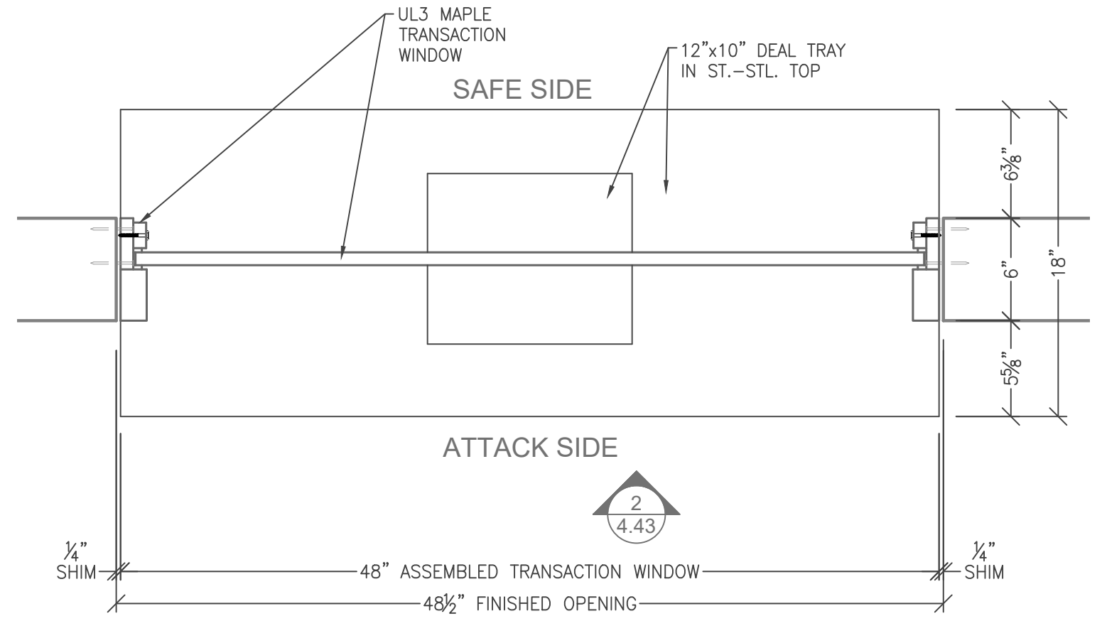
1 4.43 UL3 TRANSACTION WINDOW NATURAL VOICE TW-NV-4030-MAP18-UL03 SCALE: 1-1/2" = 1'-0"
