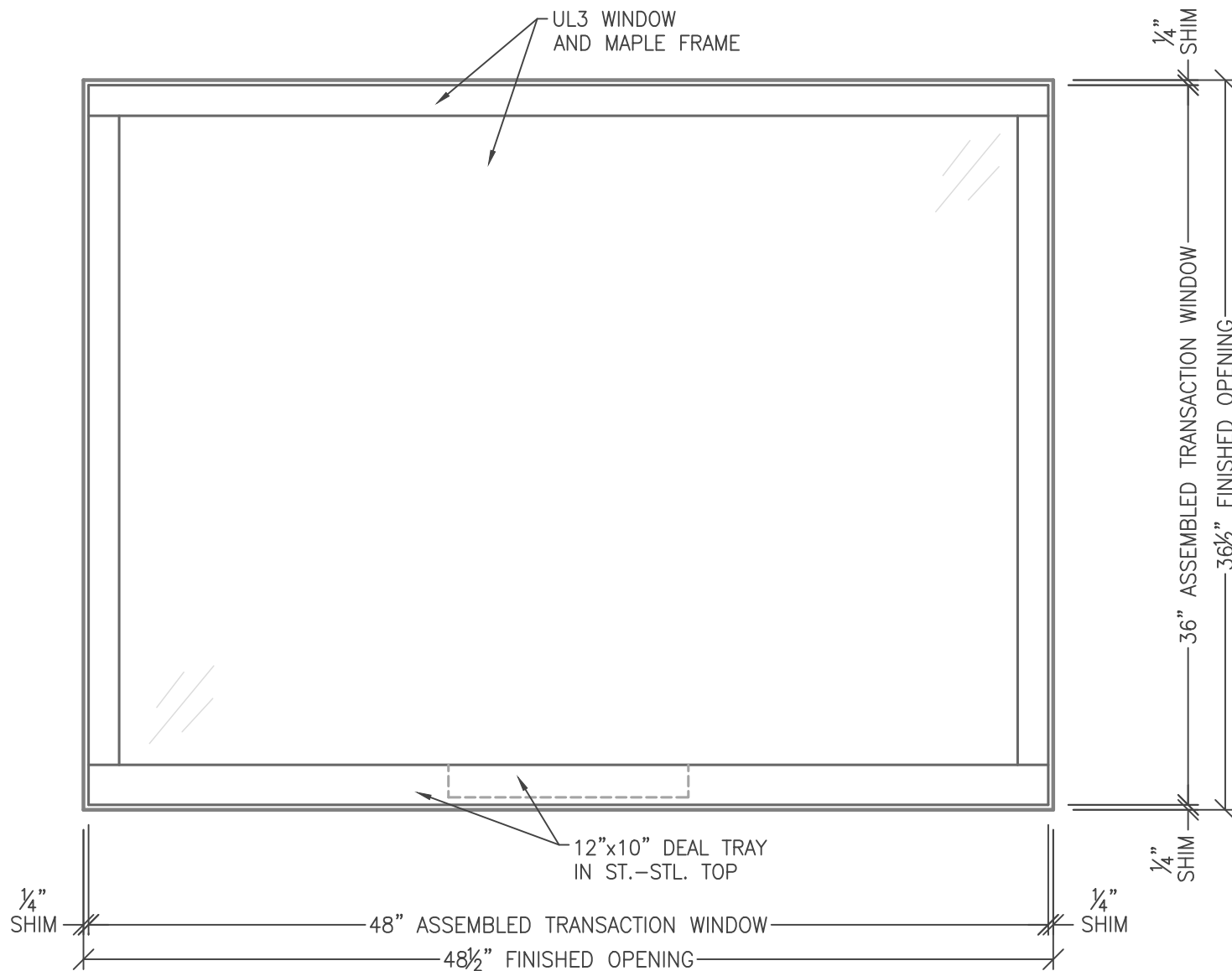
2 ATTACK SIDE ELEVATION 4.13 SCALE: 1-1/2" = 1'-0"
