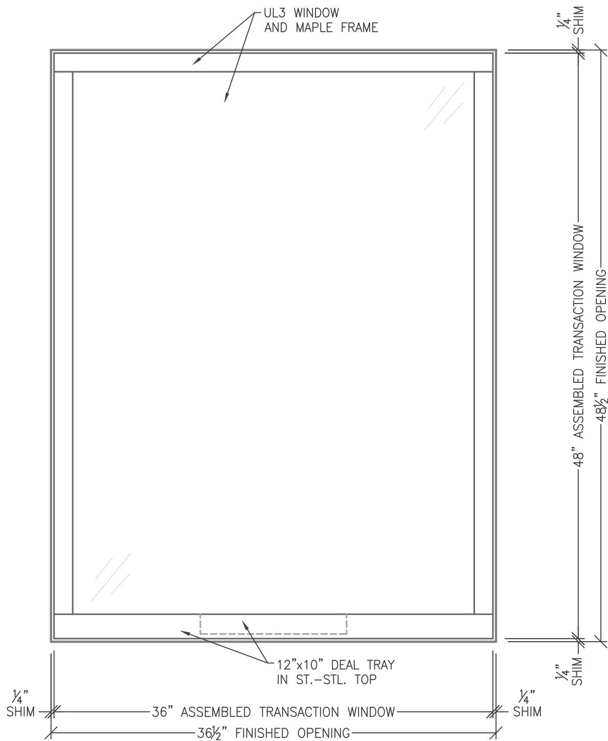
ATTACK SIDE ELEVATION 2 4.14 SCALE: 1-1/2" = 1'-0"
