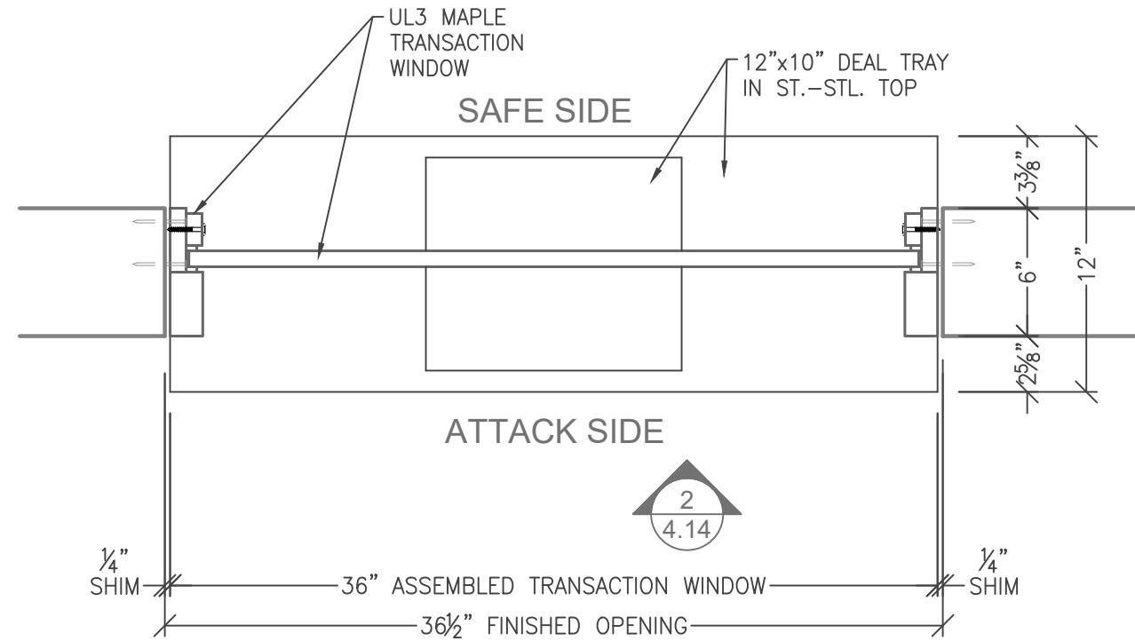
UL3 TRANSACTION WINDOW NATURAL VOICE TW-NV-3040-MAP12-UL03 1 4.14 SCALE: 1-1/2" = 1'-0"
