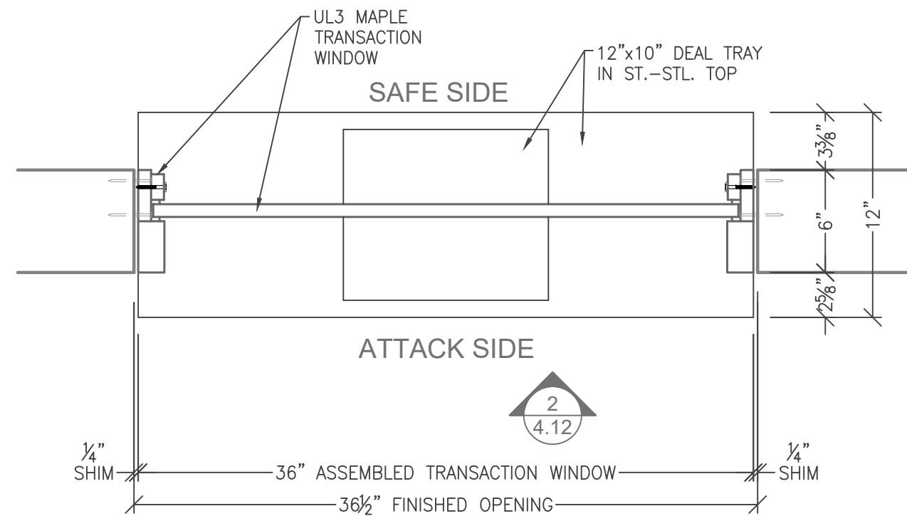
UL3 TRANSACTION WINDOW NATURAL VOICE TW-NV-3030-MAP12-UL03 1 4.12 SCALE: 1-1/2" = 1'-0"
