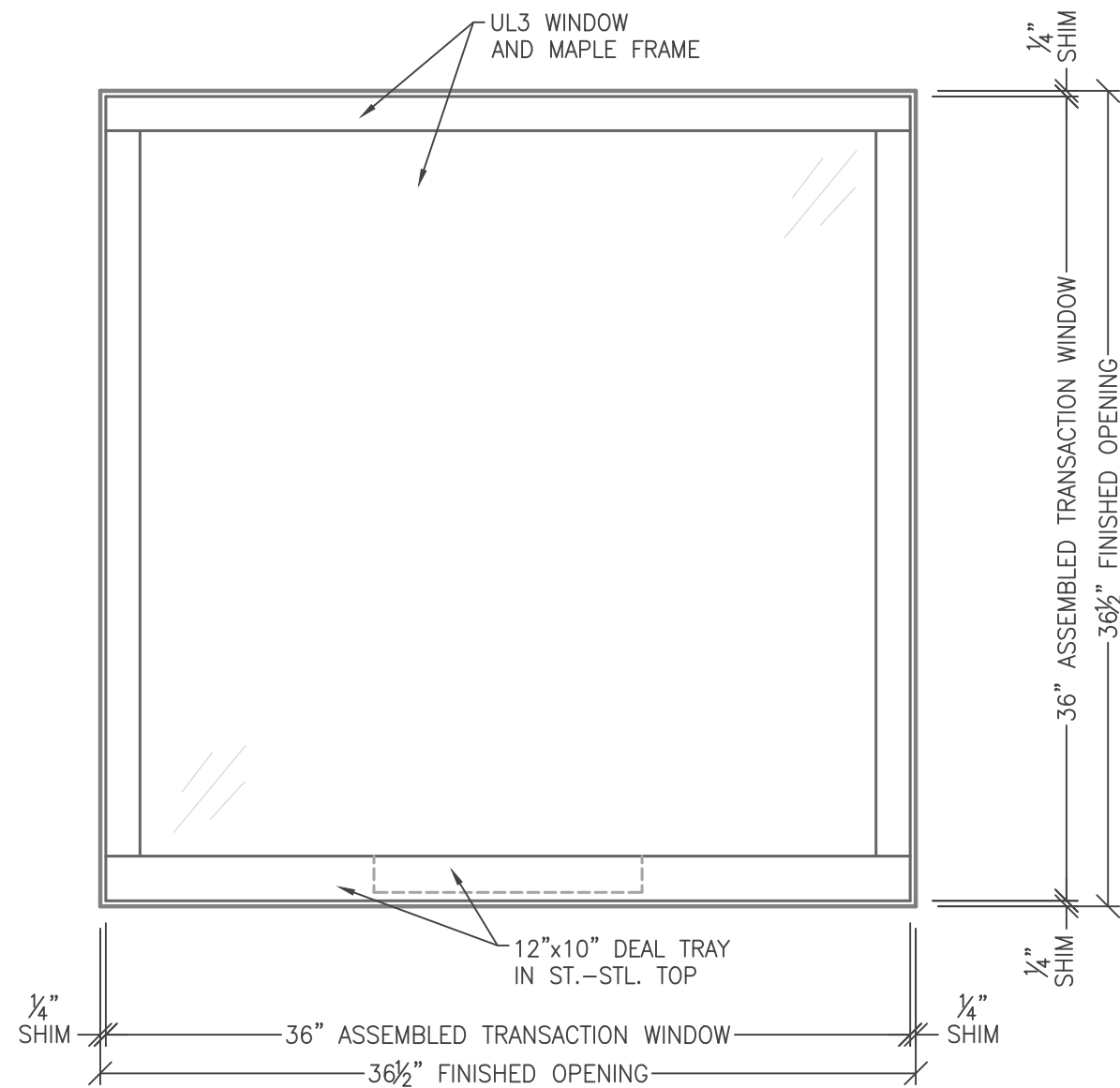
ATTACK SIDE ELEVATION 2 4.12 SCALE: 1-1/2" = 1'-0"
