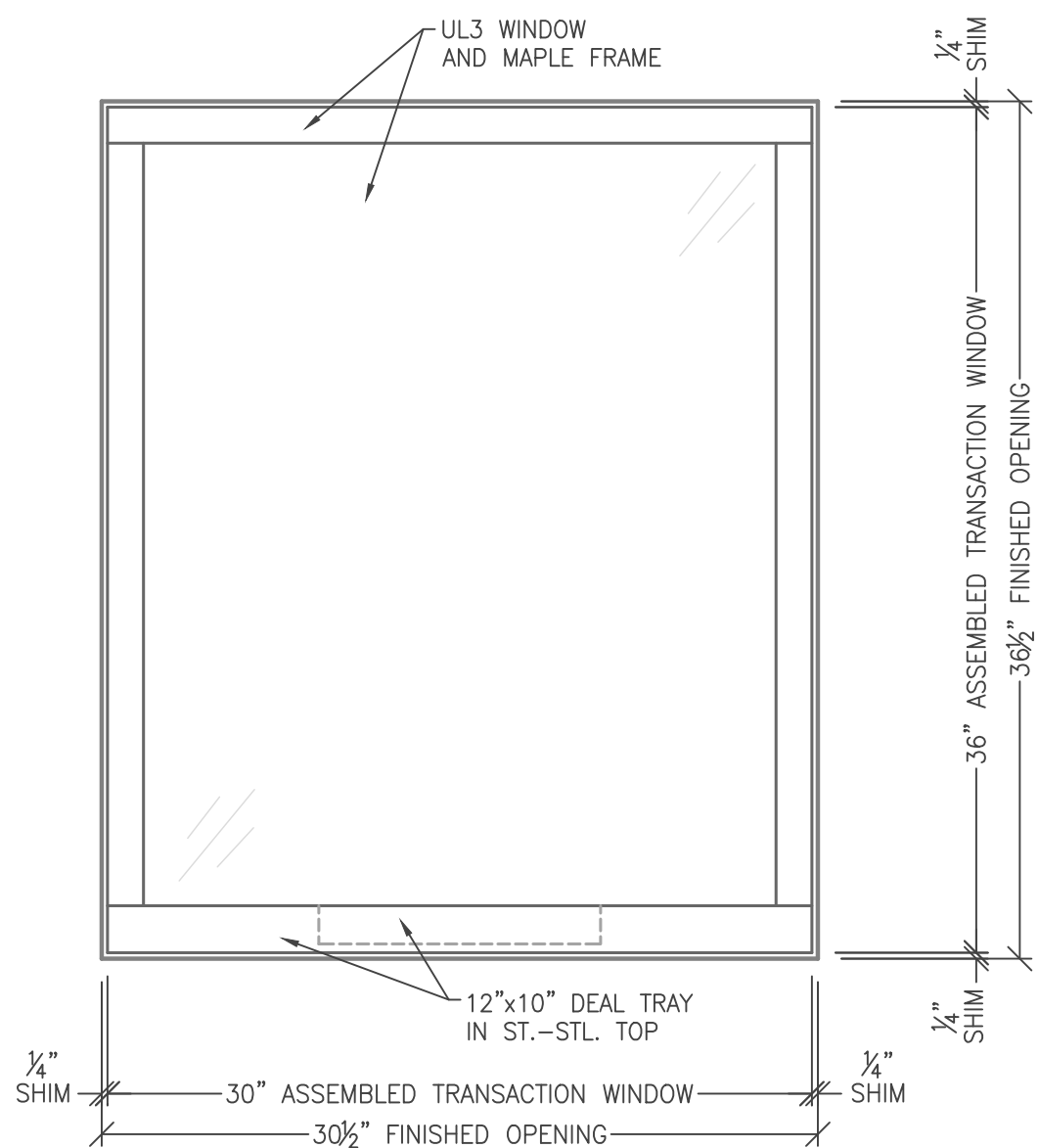
2 4.41 ATTACK SIDE ELEVATION SCALE: 1-1/2" = 1'-0"
