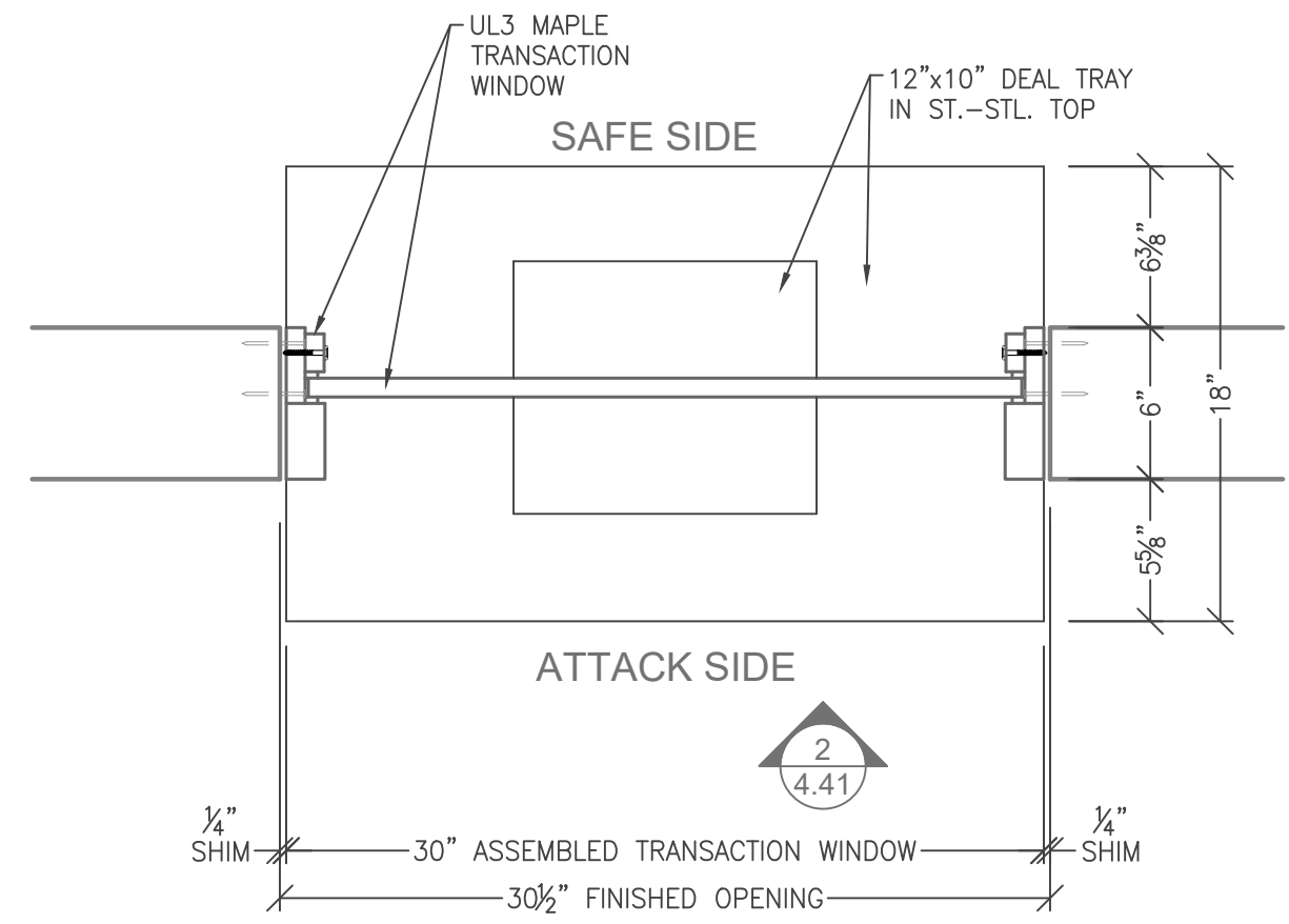
1 4.41 UL3 TRANSACTION WINDOW NATURAL VOICE TW-NV-2630-MAP18-UL03 SCALE: 1-1/2" = 1'-0"
