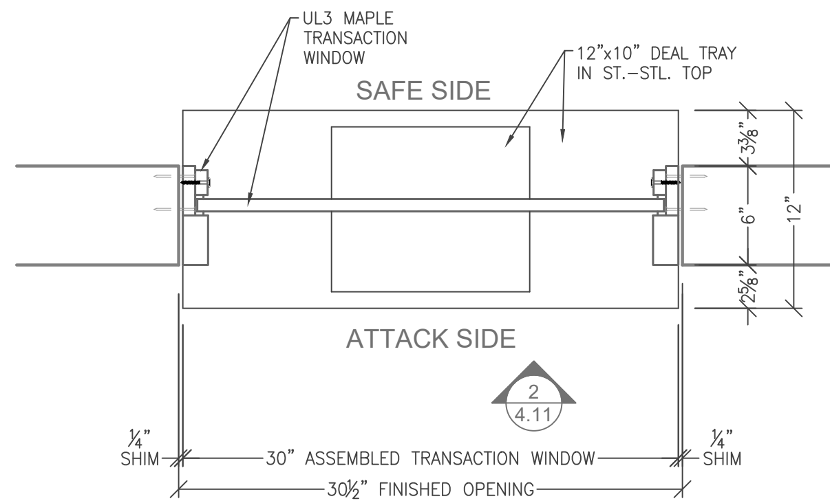
1 4.11 UL3 TRANSACTION WINDOW NATURAL VOICE TW-NV-2630-MAP12-UL03 SCALE: 1-1/2" = 1'-0"
