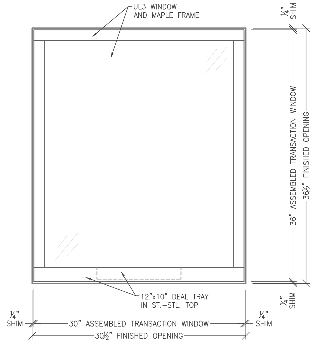
2 4.11 ATTACK SIDE ELEVATION SCALE: 1-1/2" = 1'-0"
