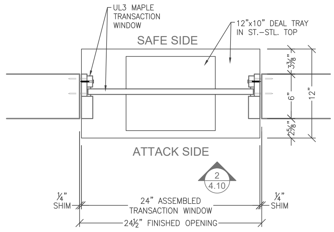
1 4.10 UL3 TRANSACTION WINDOW NATURAL VOICE TW-NV-2030-MAP12-UL03 SCALE: 1-1/2" = 1'-0"
