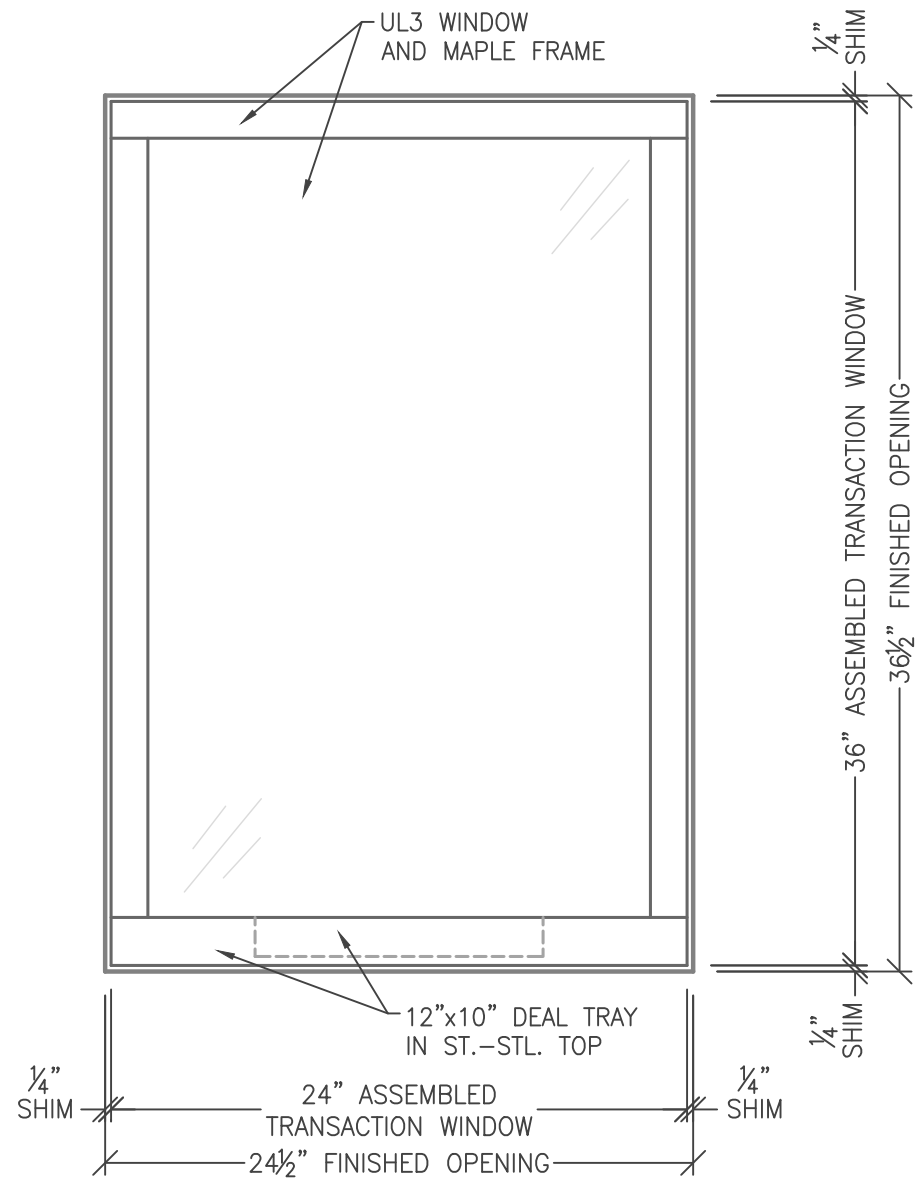
2 4.10 ATTACK SIDE ELEVATION SCALE: 1-1/2" = 1'-0"
