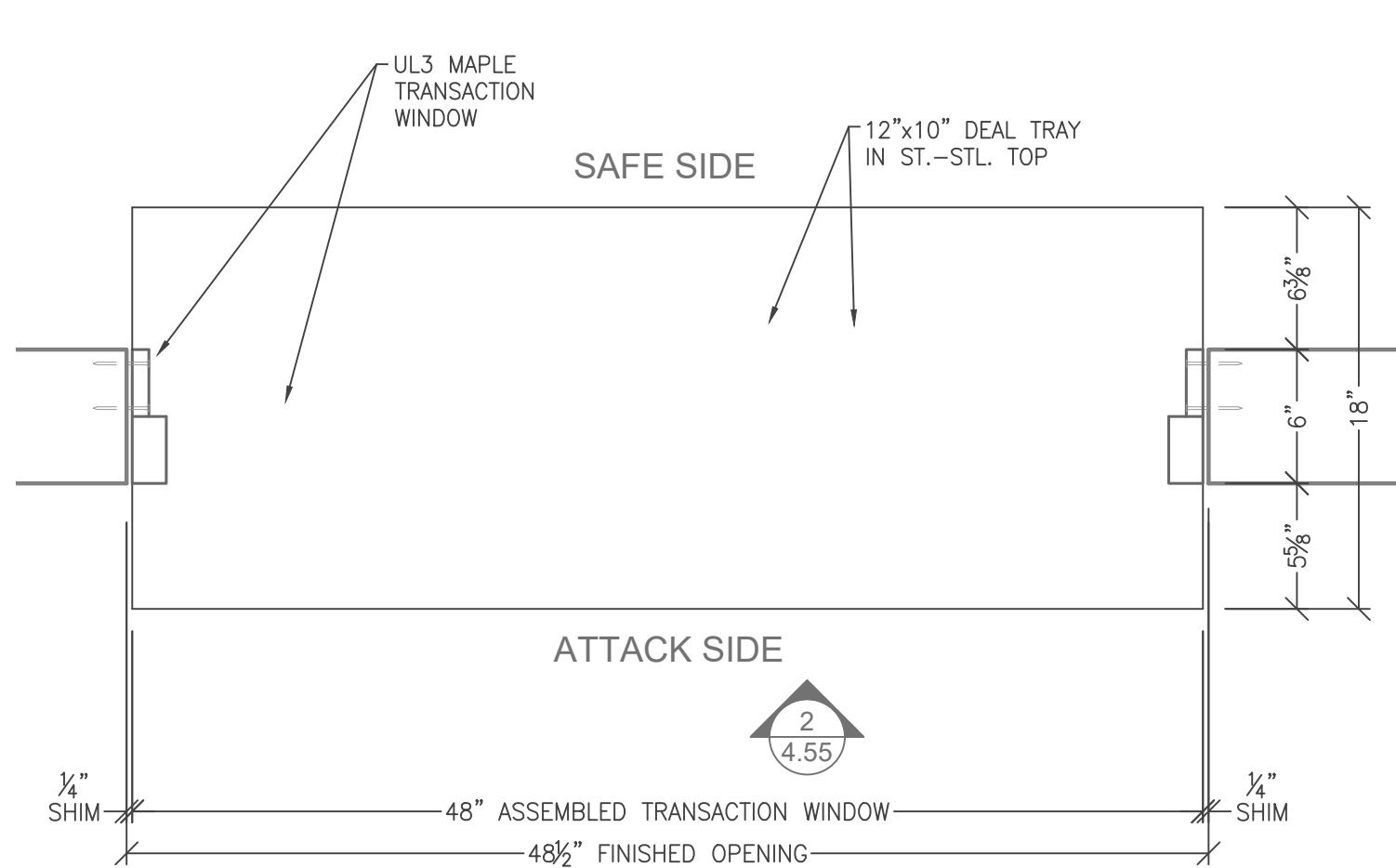
UL3 TRANSACTION WINDOW SPEAK THRU - DISK TW-DS-4040-MAP18-UL03 1 4.55 SCALE: 1-1/2" = 1'-0"
