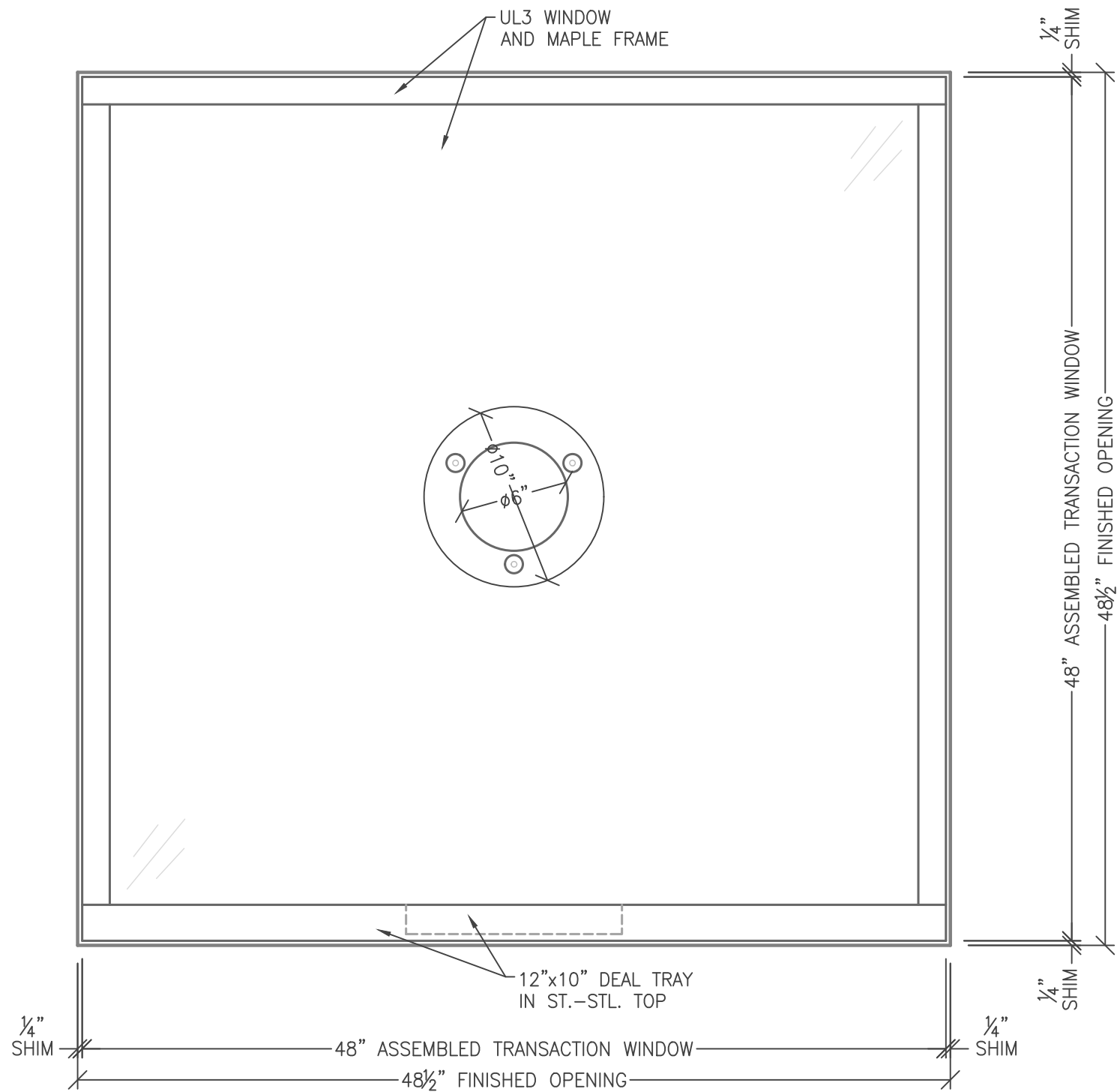
ATTACK SIDE ELEVATION 2 4.55 SCALE: 1-1/2" = 1'-0"
