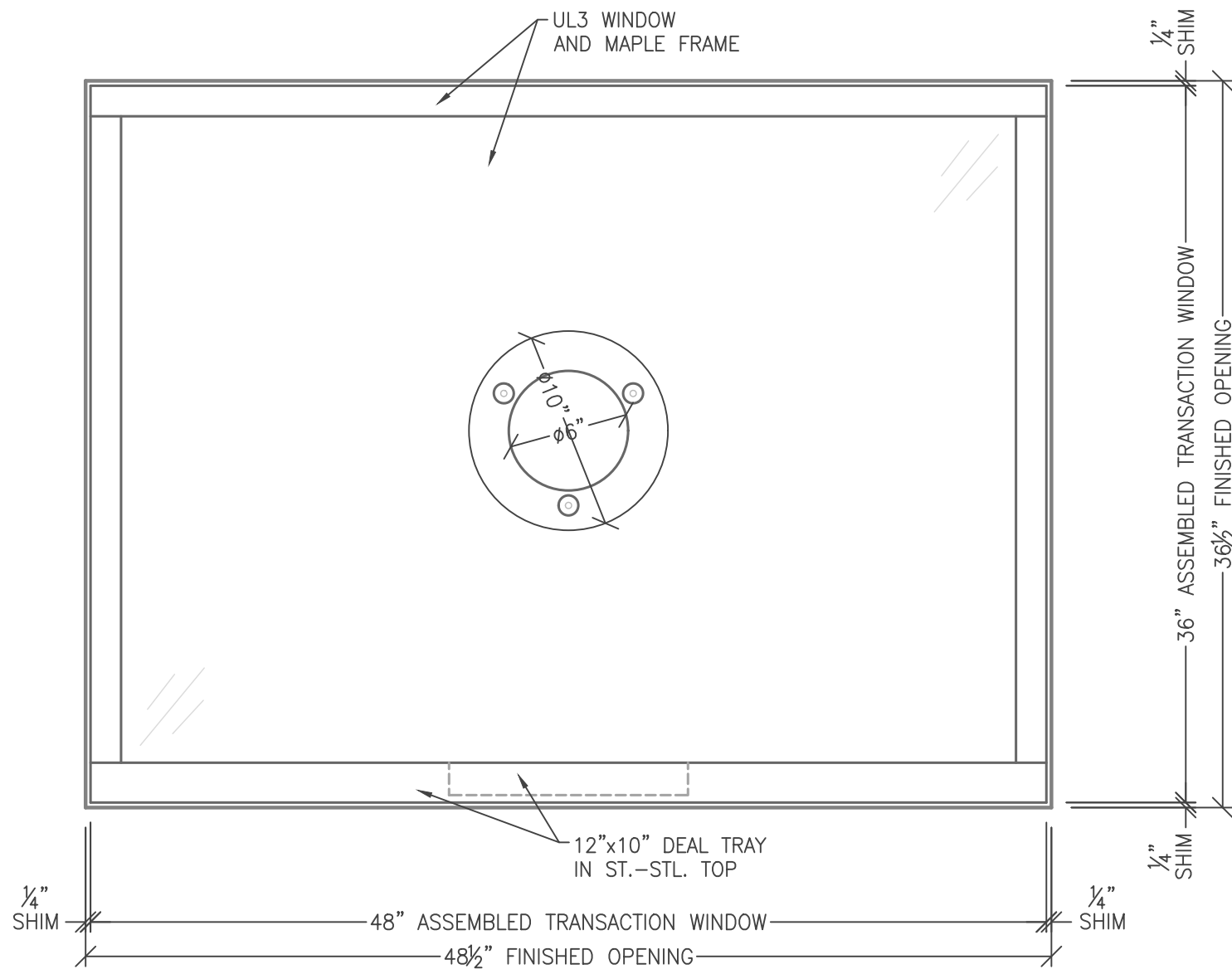
2 4.53 ATTACK SIDE ELEVATION SCALE: 1-1/2" = 1'-0"
