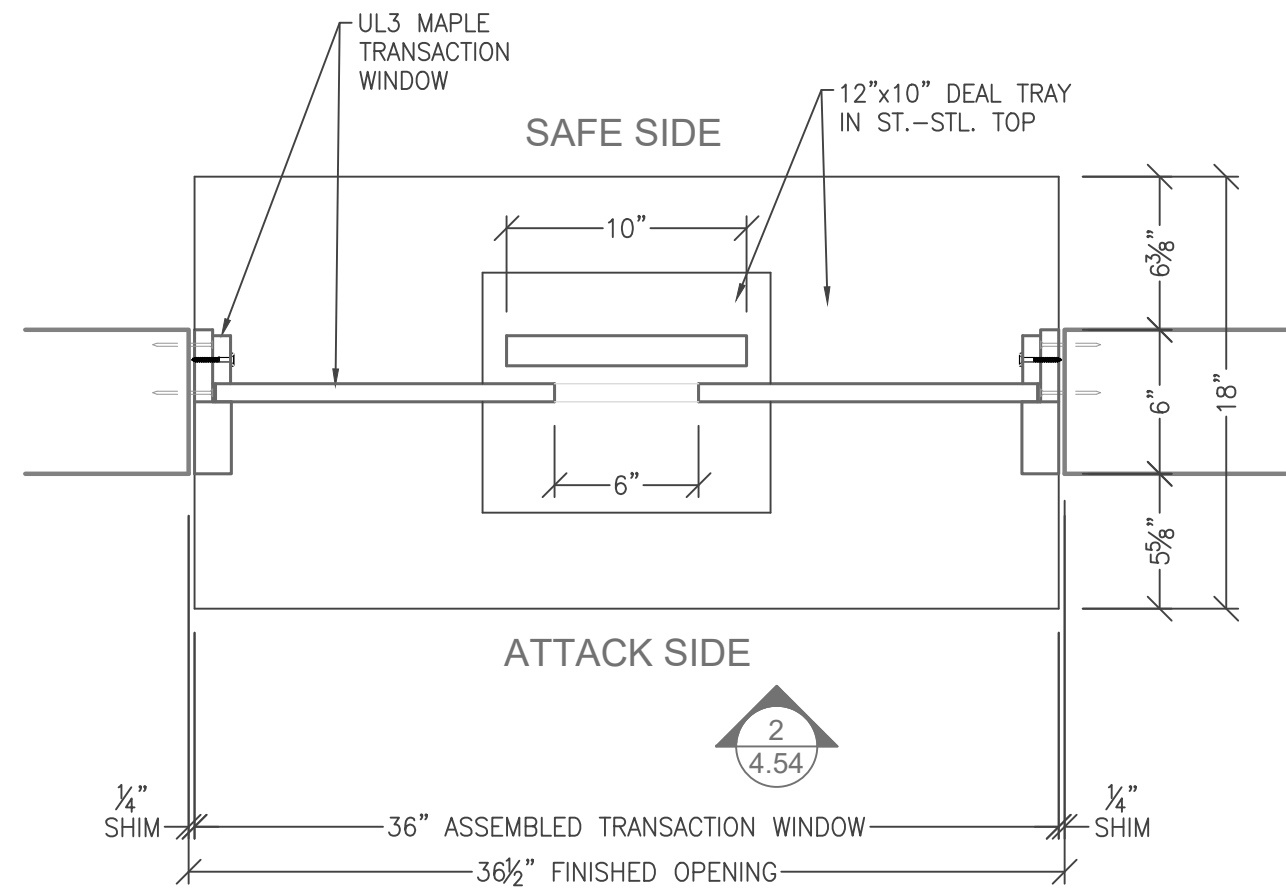
UL3 TRANSACTION WINDOW SPEAK THRU - DISK TW-DS-3040-MAP18-UL03 1 4.54 SCALE: 1-1/2" = 1'-0"
