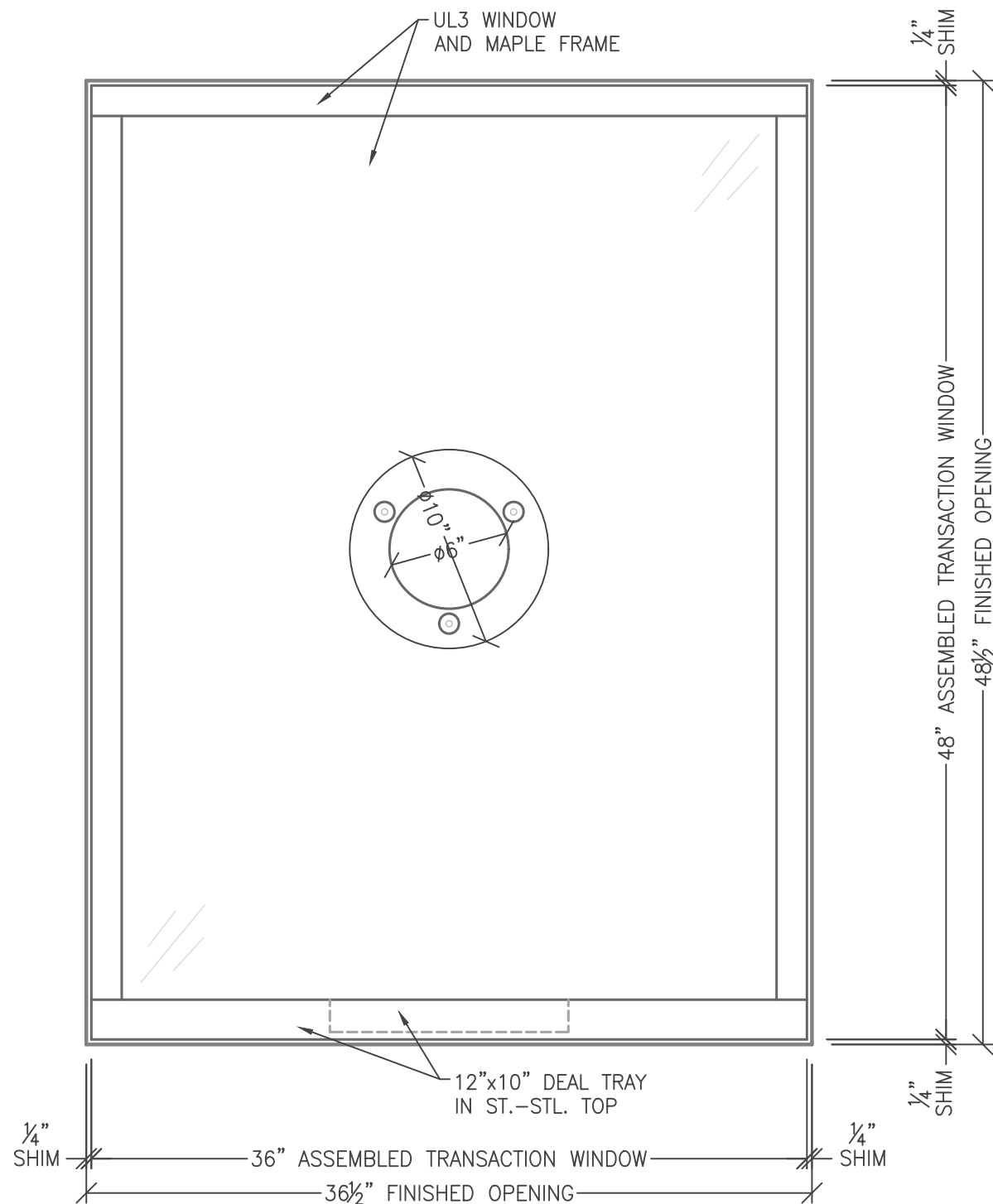
ATTACK SIDE ELEVATION 2 4.54 SCALE: 1-1/2" = 1'-0"
