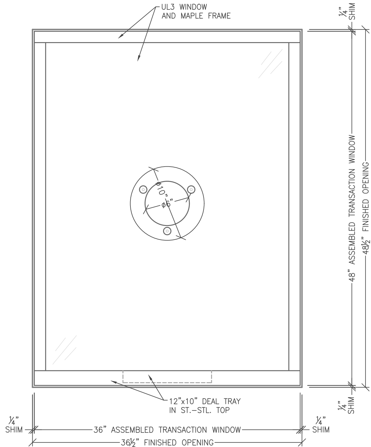
ATTACK SIDE ELEVATION 2 4.24 SCALE: 1-1/2" = 1'-0"
