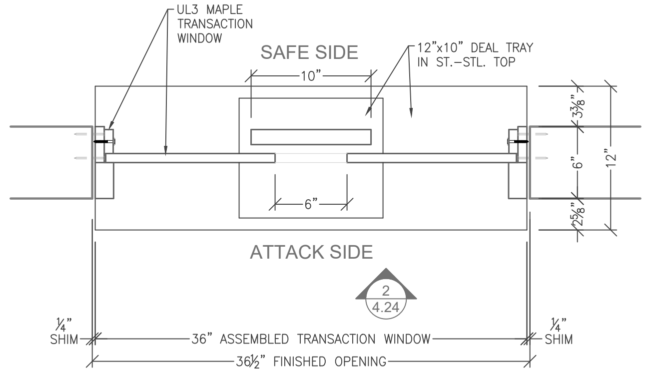
UL3 TRANSACTION WINDOW SPEAK THRU - DISK TW-DS-3040-MAP12-UL03 1 4.24 SCALE: 1-1/2" = 1'-0"
