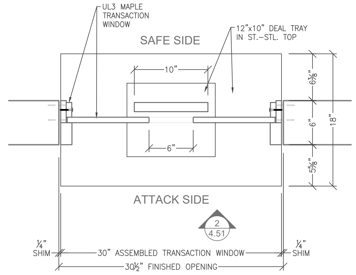
UL3 TRANSACTION WINDOW SPEAK THRU - DISK TW-DS-2630-MAP18-UL03 1 4.51 SCALE: 1-1/2" = 1'-0"
