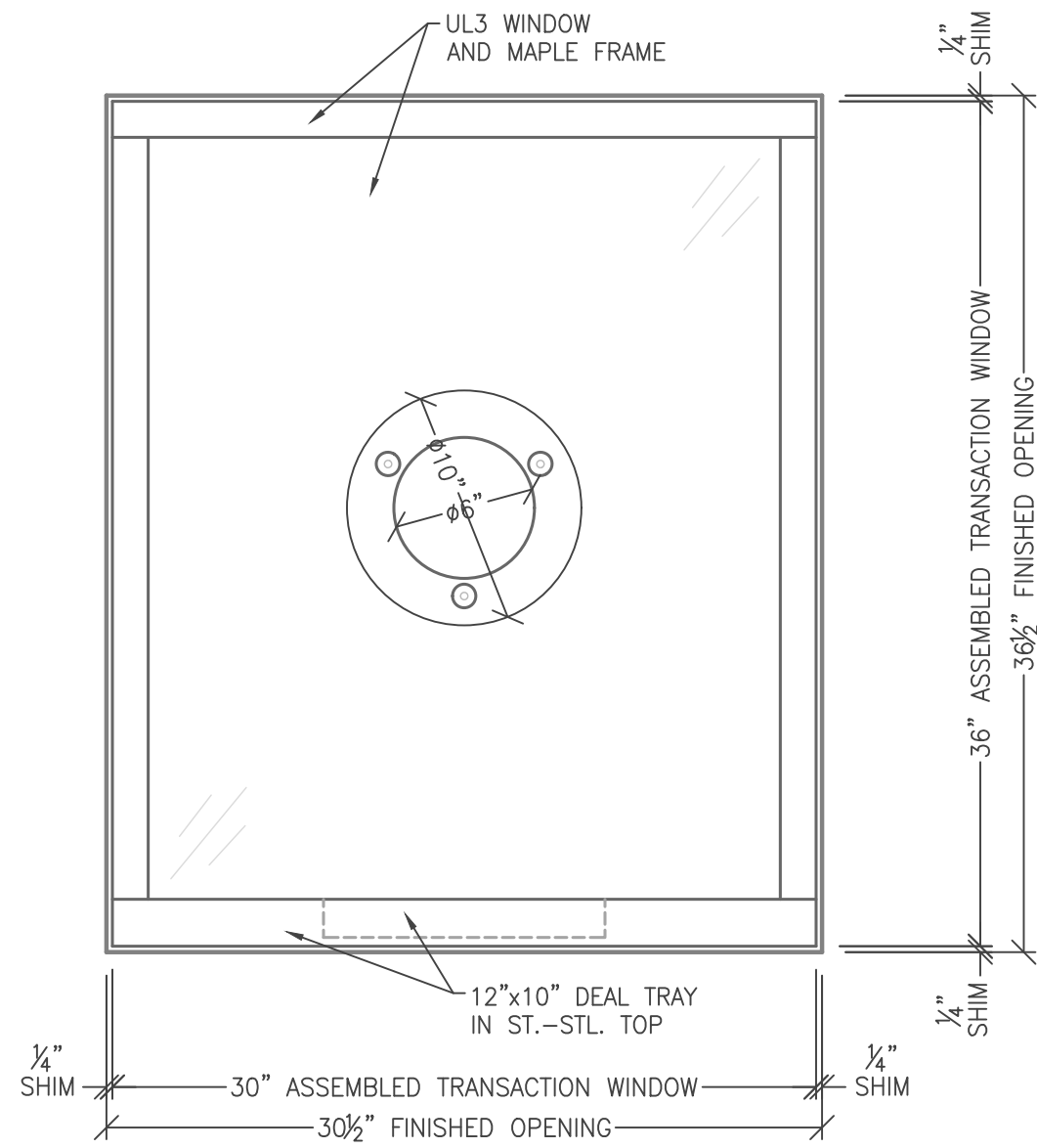
ATTACK SIDE ELEVATION 2 4.51 SCALE: 1-1/2" = 1'-0"
