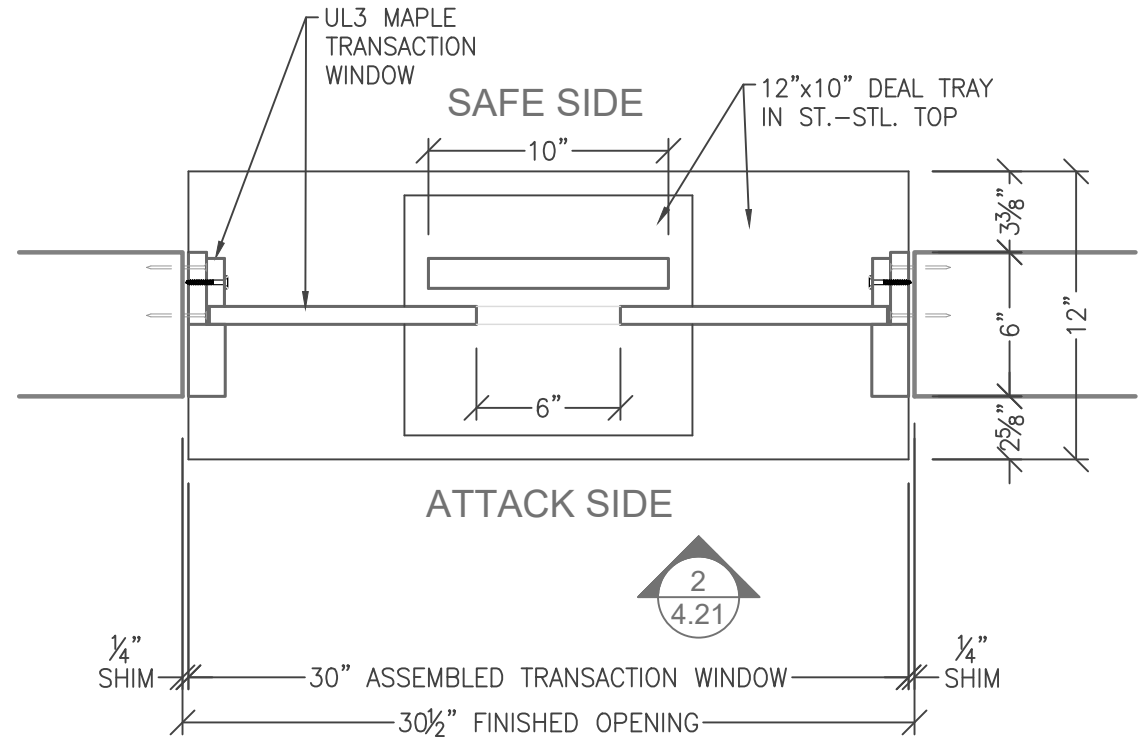
1 4.21 UL3 TRANSACTION WINDOW SPEAK THRU - DISK TW-DS-2630-MAP12-UL03 SCALE: 1-1/2" = 1'-0"
