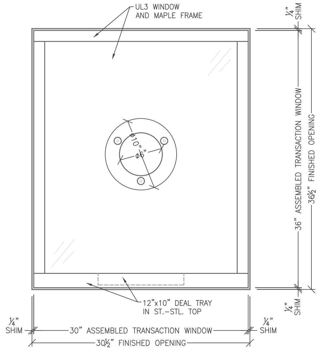
2 4.21 ATTACK SIDE ELEVATION SCALE: 1-1/2" = 1'-0"
