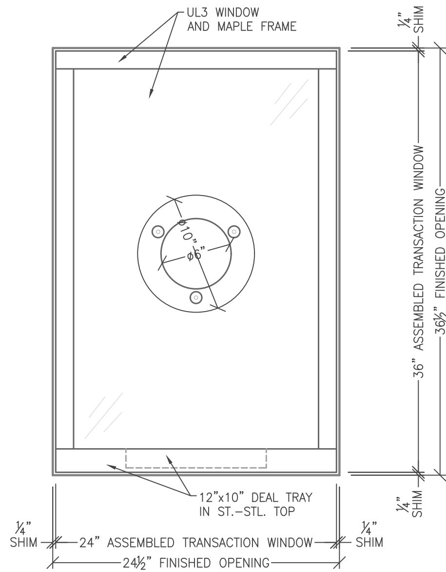
ATTACK SIDE ELEVATION 2 4.50 SCALE: 1-1/2" = 1'-0"
