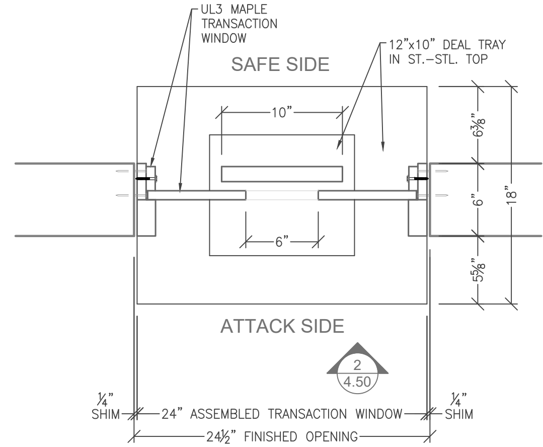
UL3 TRANSACTION WINDOW SPEAK THRU - DISK TW-DS-2030-MAP18-UL03 1 4.50 SCALE: 1-1/2" = 1'-0"
