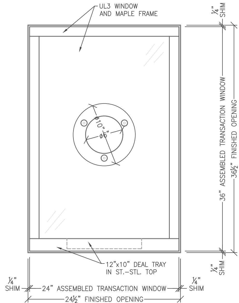
ATTACK SIDE ELEVATION 2 4.20 SCALE: 1-1/2" = 1'-0"
