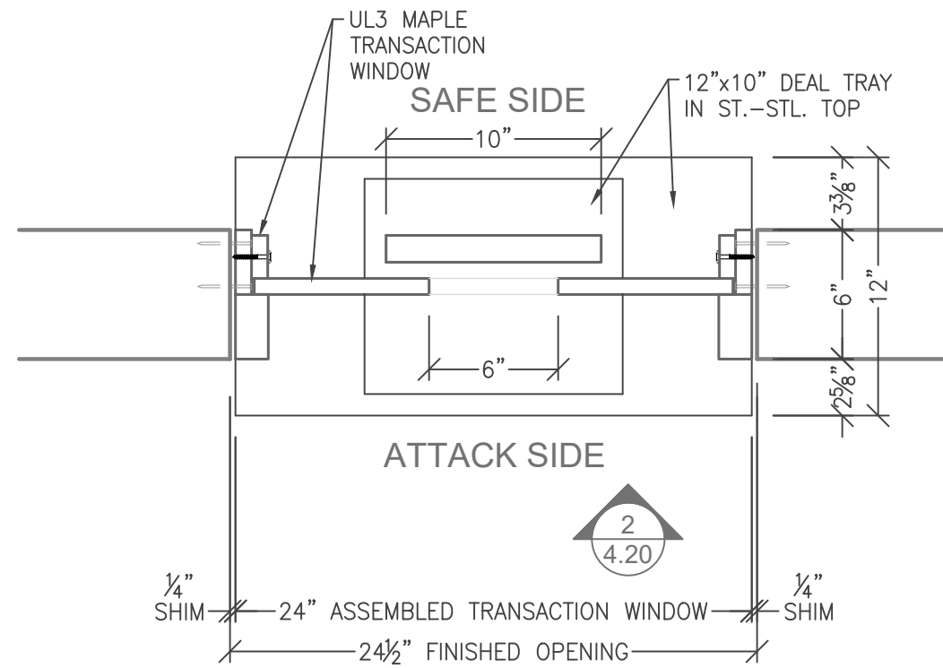
UL3 TRANSACTION WINDOW SPEAK THRU - DISK TW-DS-2030-MAP12-UL03 1 4.20 SCALE: 1-1/2" = 1'-0"
