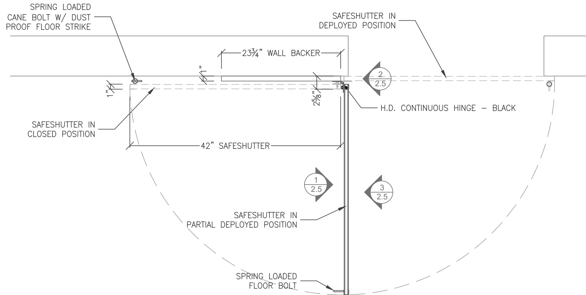
1 2.4 UL3 SAFESHUTTER SS-WB-3660-WHWHI-UL03 SCALE: 1" = 1'-0"
