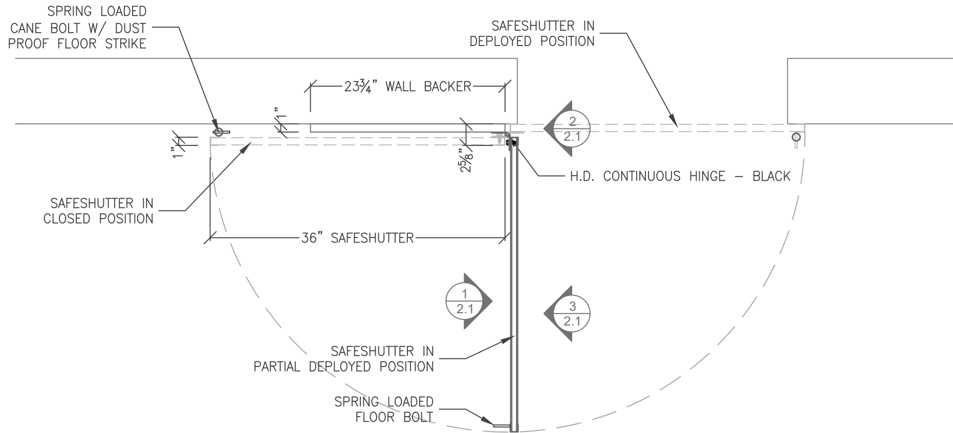
UL3 SAFESHUTTER 1 SS-WB-3060-WHWHI-UL03 2.0 SCALE: 1" = 1'-0"
