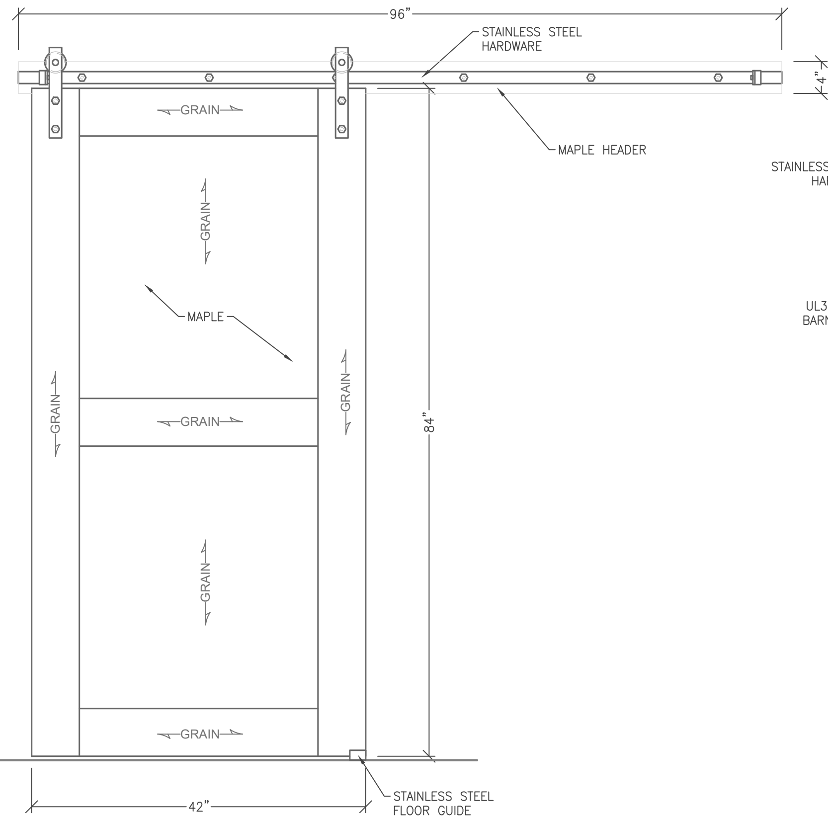
1 3.0 UL3 B.R. BARN DOOR BD-2P-3670-MAPSS-UL03 SCALE: 1" = 1'-0"
